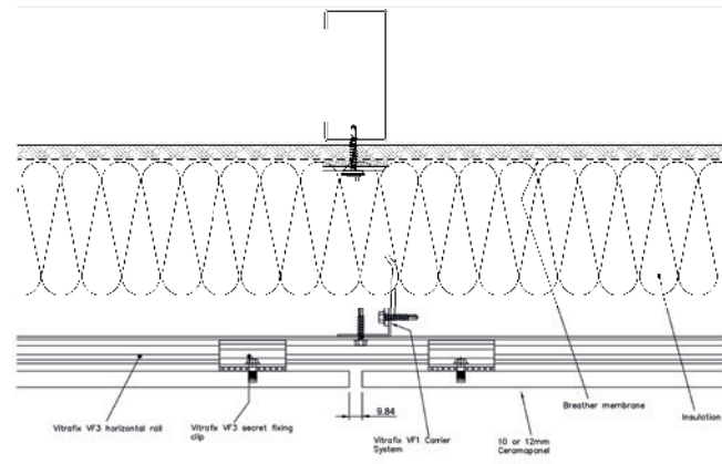
CERMAPANEL® VITRAFIX VF3 VERTICAL JOINT
