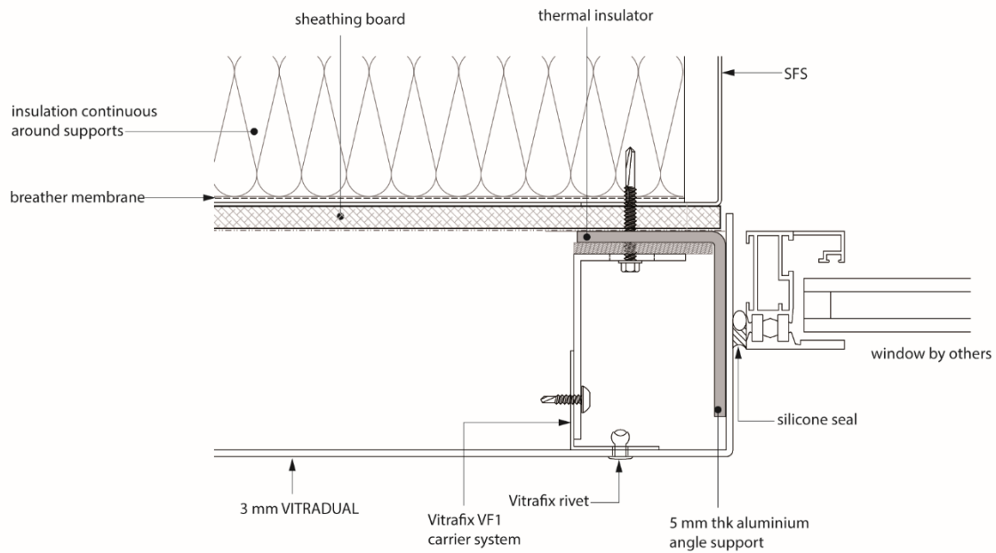
Figure 1 Typical installation details (continued)
