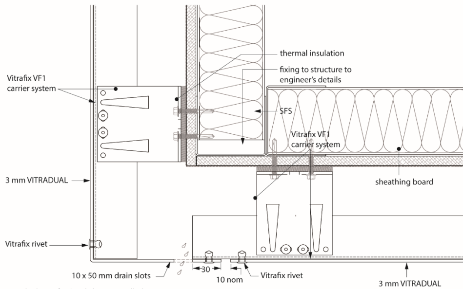
Figure 1 Typical installation details (continued)
